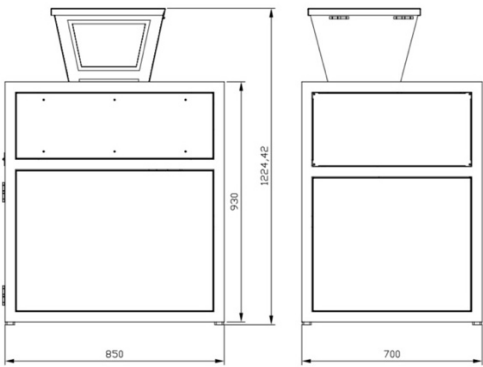
Fig. 4: L×W×H (mm) Fits through office doors and elevators
