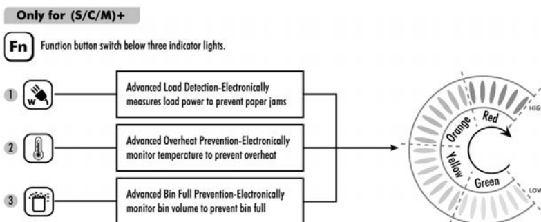
Fig. 4: Control Panel View (Panel with dynamic load display)
